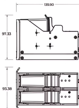
REACHe Printhead (Stitched) — 135.90mm (W) × 97.33mm (H) × 93.38mm (D)
